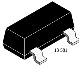
BFS17A Marking: E2 Plastic case (SOT 23) 1 = Collector, 2 = Base, 3 = Emitter
