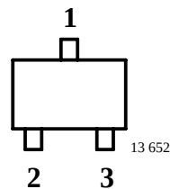
BFS17AW Marking: WE2 Plastic case (SOT 323) 1 = Collector, 2 = Base, 3 = Emitter
