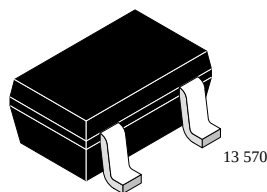
BFS17AW Marking: WE2 Plastic case (SOT 323) 1 = Collector, 2 = Base, 3 = Emitter
