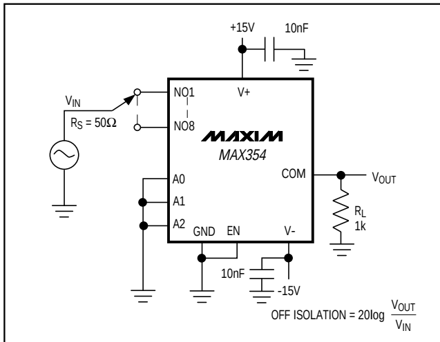
Figure 5. Off Isolation
