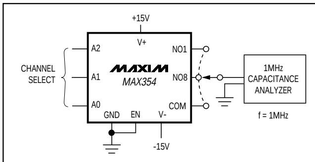
Figure 7. NO/COM Capacitance
