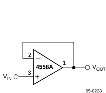
Figure 18. Voltage Follower
