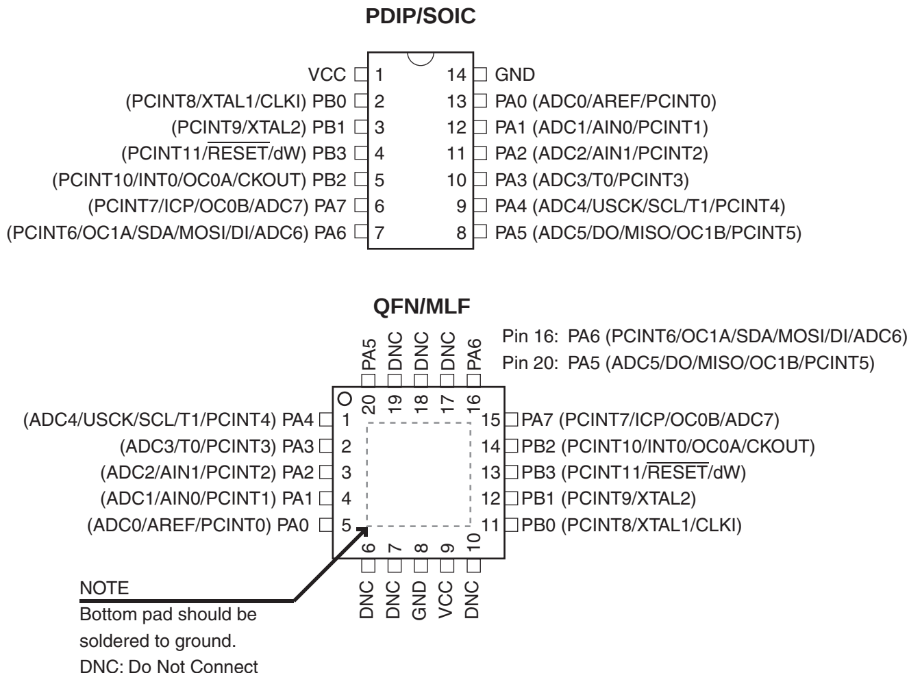
Figure 1-1. Pinout ATtiny24/44/84
