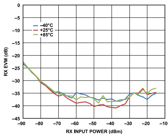
Figure 7. RX EVM vs. RX Input Power, GSM Mode, 30.72 MHz REF_CLK (Doubled Internally for RF Synthesizer)
