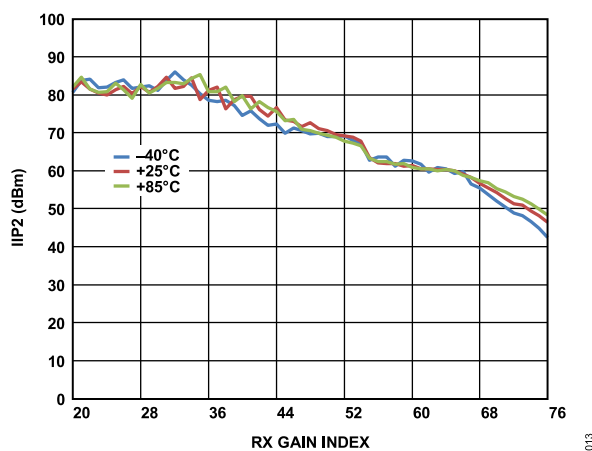
Figure 13. Second-Order Input Intercept Point (IIP2) vs. RX Gain Index, f_1 = 2.00 MHz, f_2 = 2.01 MHz, GSM Mode
