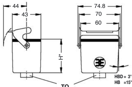
KVL
