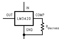
Figure 13. Changing V_{REG}
