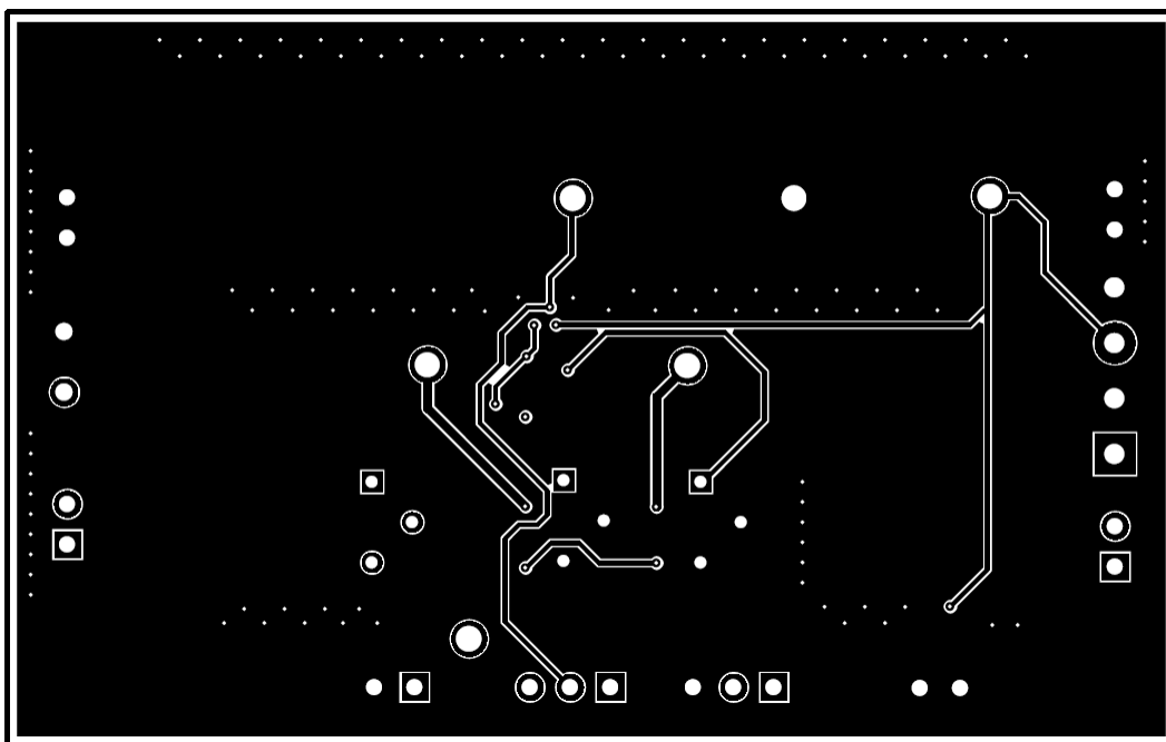
Figure 7. Bottom Layer
