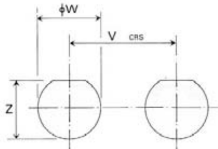
PANEL CUT-OUT DETAILS
