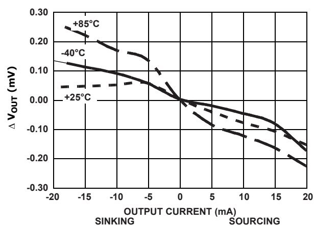
FIGURE 11. LOAD REGULATION
