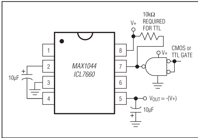
Figure 7. External Clocking
