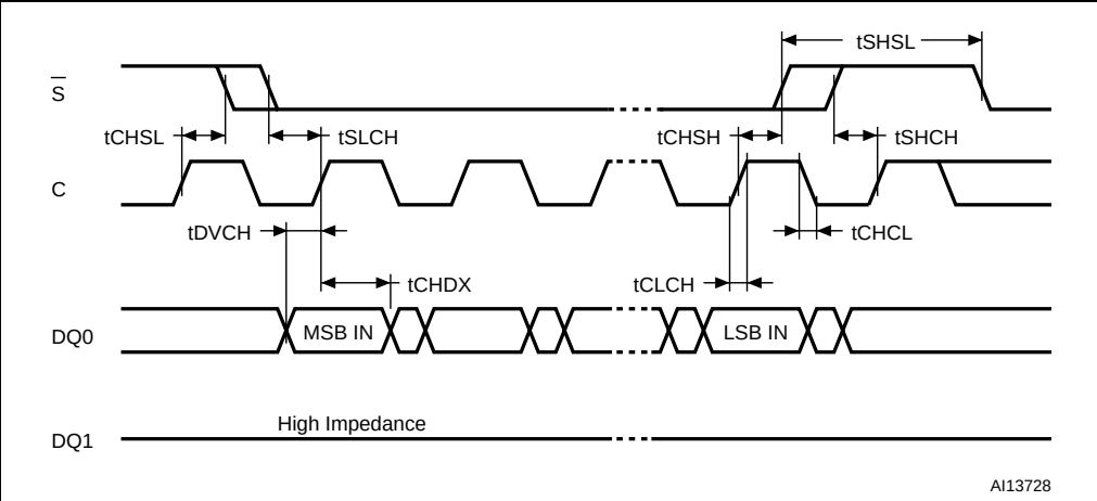
Figure 103. Serial input timing
