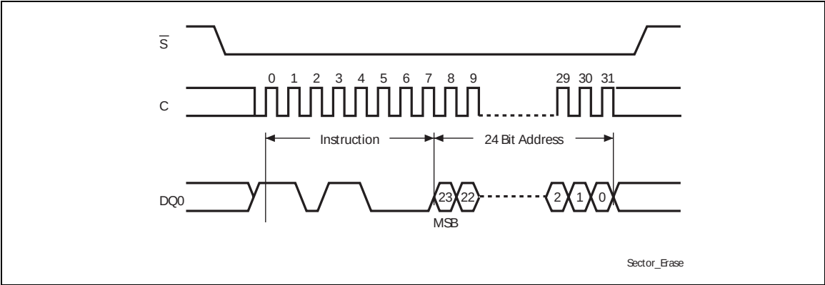
Figure 28. Sector Erase instruction sequence
