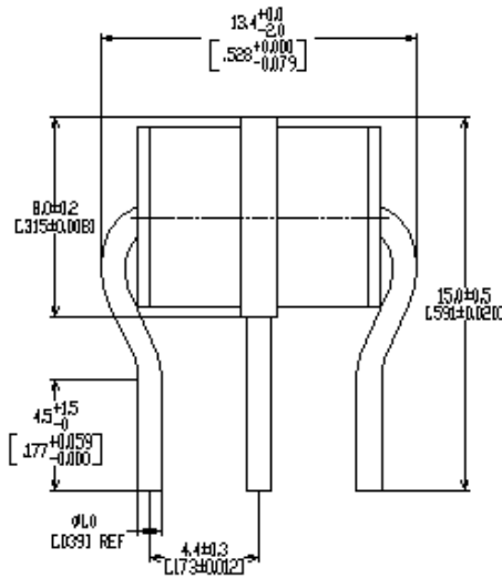
Axial Leaded (GTCA38-XXXM-R10)
