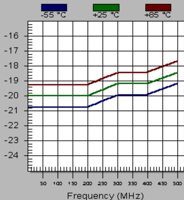
TM6505 Reverse Isolation (dB)
