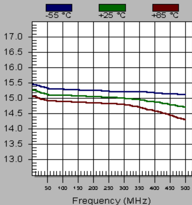
TM6505 Gain (dB)
