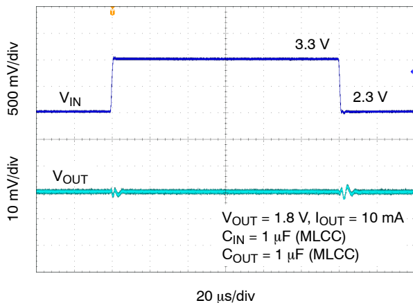
Figure 30. Line Transient Response – V_{OUT} = 1.8 V
