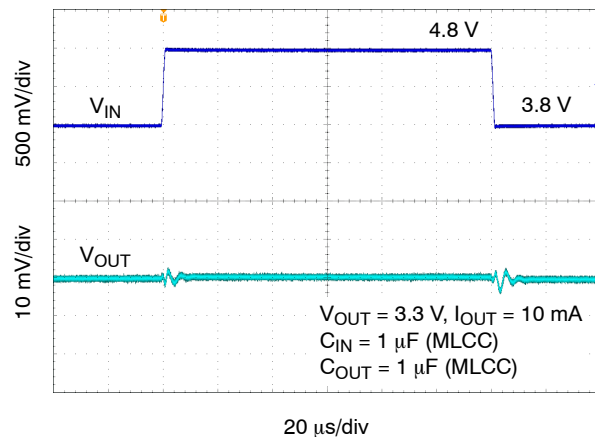
Figure 31. Line Transient Response – V_{OUT} = 3.3 V
