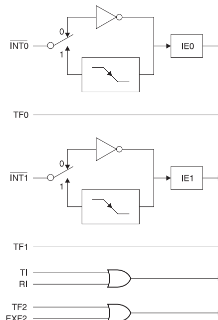
Figure 6. Interrupt Sources
