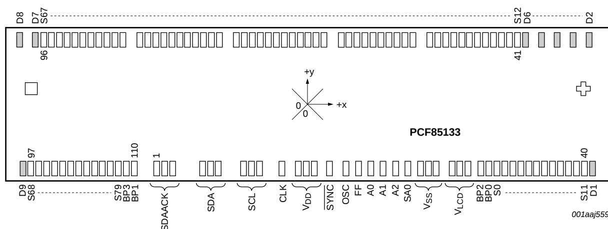
Fig 2. Pin configuration for PCF85133
