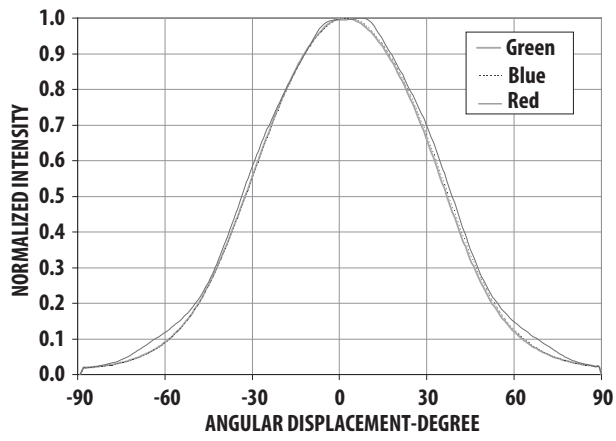
Figure 10. Radiation Pattern-Major Axis
