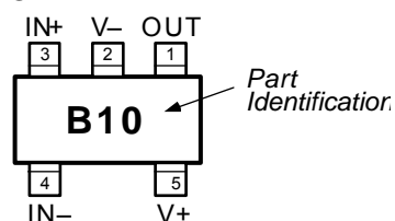
5-Pin SOT-23 (M5)
