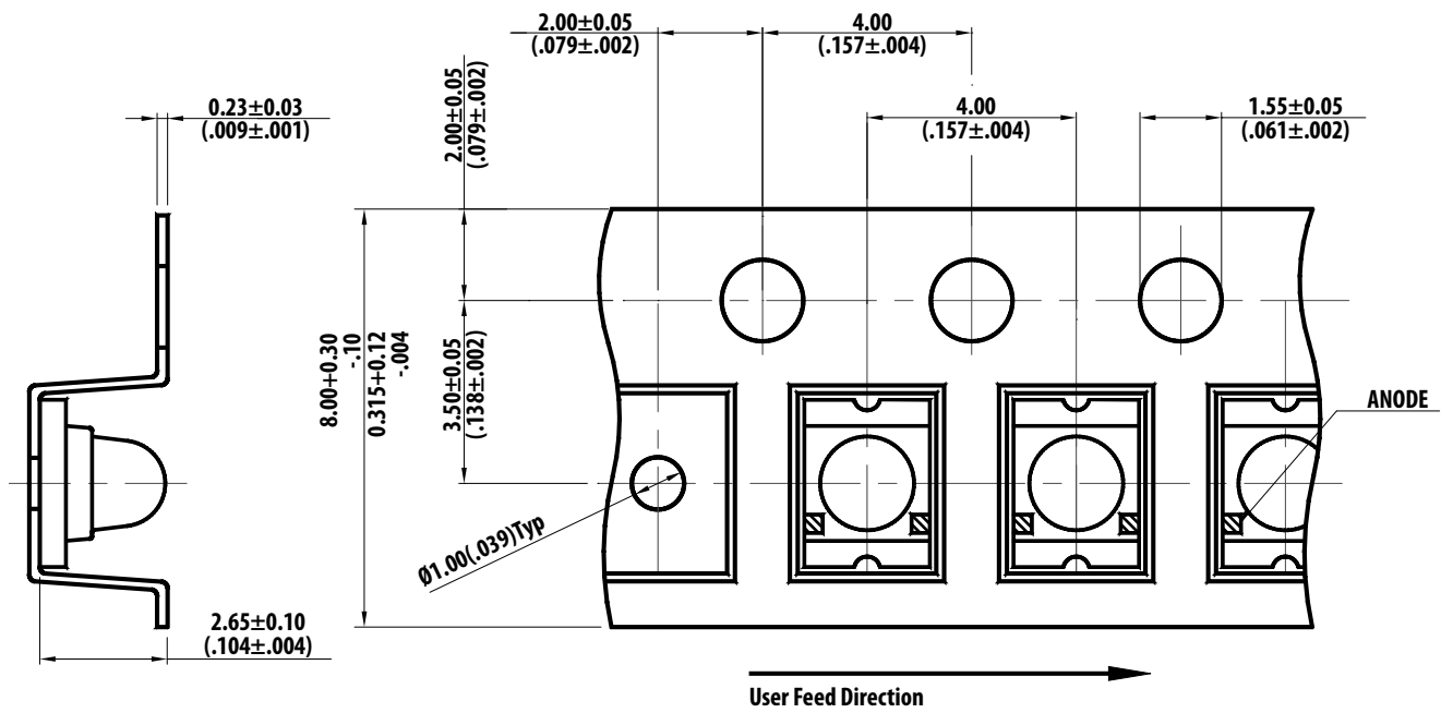
Figure 10. Tape Dimensions
