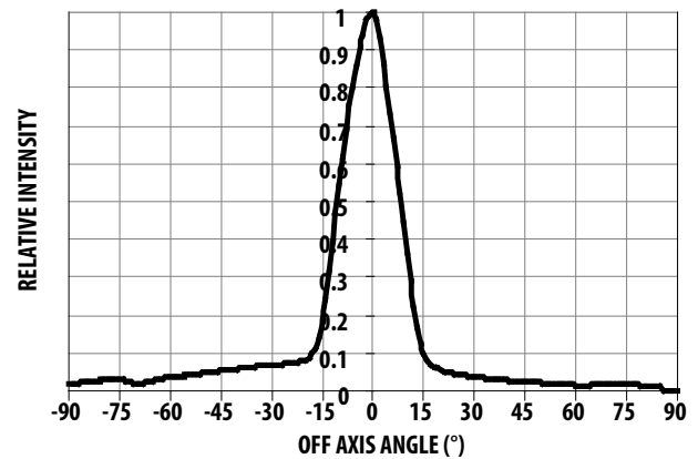
Figure 4. Vertical Radiation Pattern
