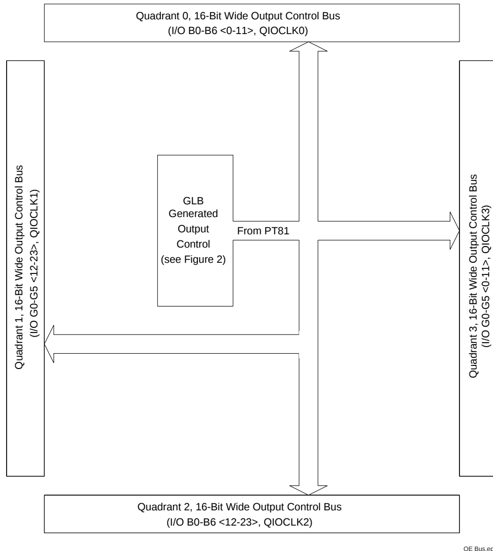
Figure 5. Output Control Bus and Quadrant Organization
