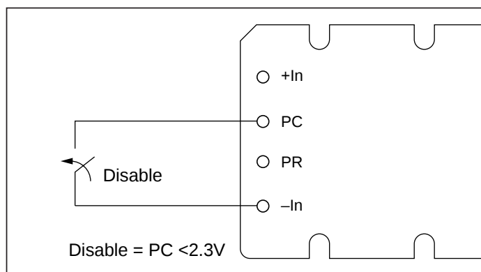
Figure 1—Module enable/disable.
