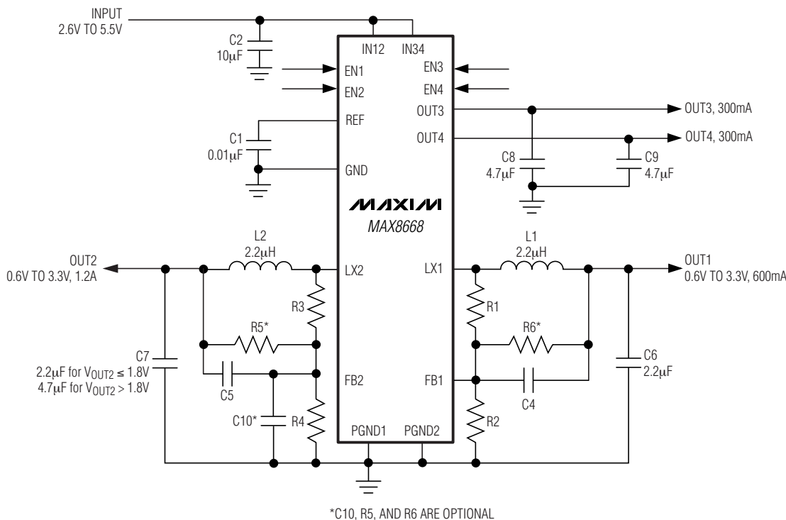
Figure 4. MAX8668 Typical Application Circuit
