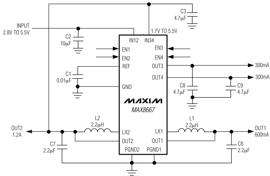
Figure 3. MAX8667 Typical Application Circuit
