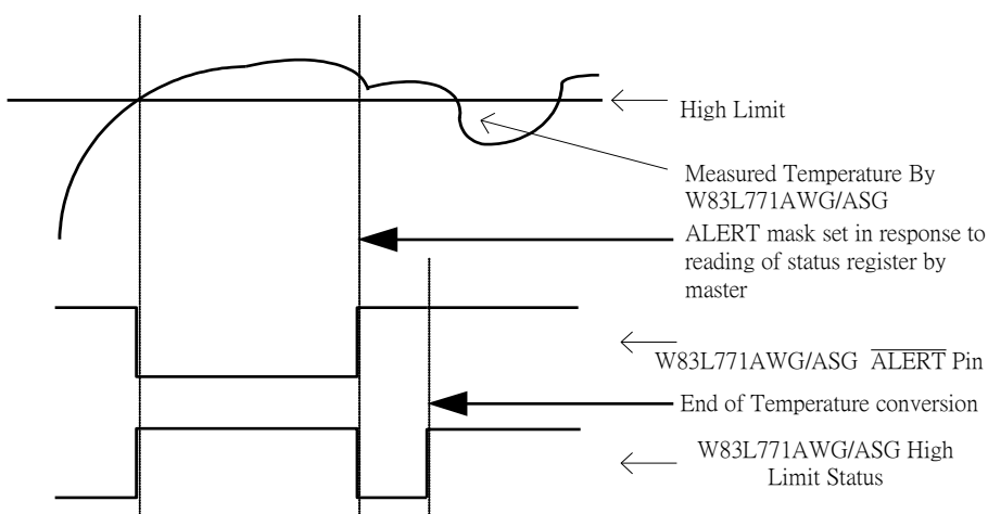
Fig. 7.3.2 Response of \overline{ALERT} output interrupt mode
