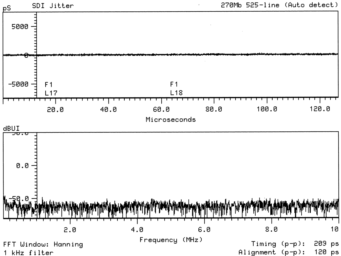
Figure 13. Jitter Plots
