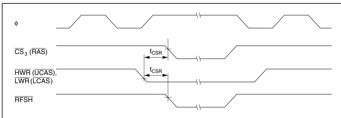
Figure 21.15 DRAM Bus Timing (Self-Refresh Mode) — 2\overline{CAS} Mode —
