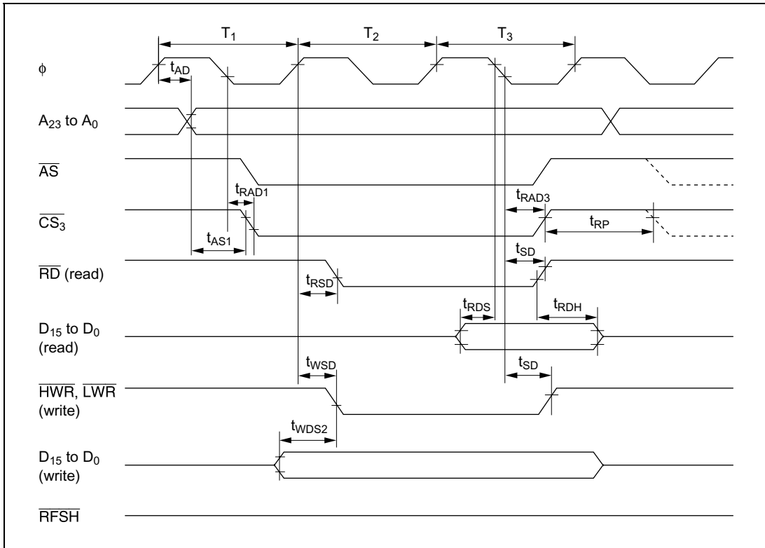
Figure 21.16 PSRAM Bus Timing (Read/Write): Three-State Access
