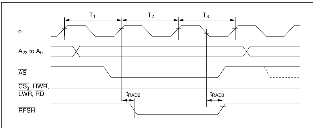
Figure 21.17 PSRAM Bus Timing (Refresh Cycle): Three-State Access
