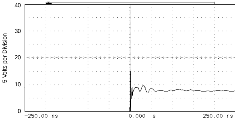
FIGURE 5 OVERSHOOT & CLAMPING VOLTAGE FOR P0402FC05C
