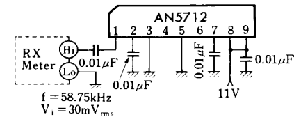
Test Circuit 2 (R i , C i )
