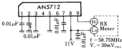
Test Circuit 3 (C O )
