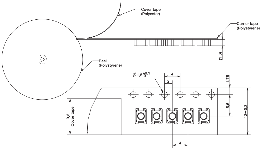
CARRIER TAPE
