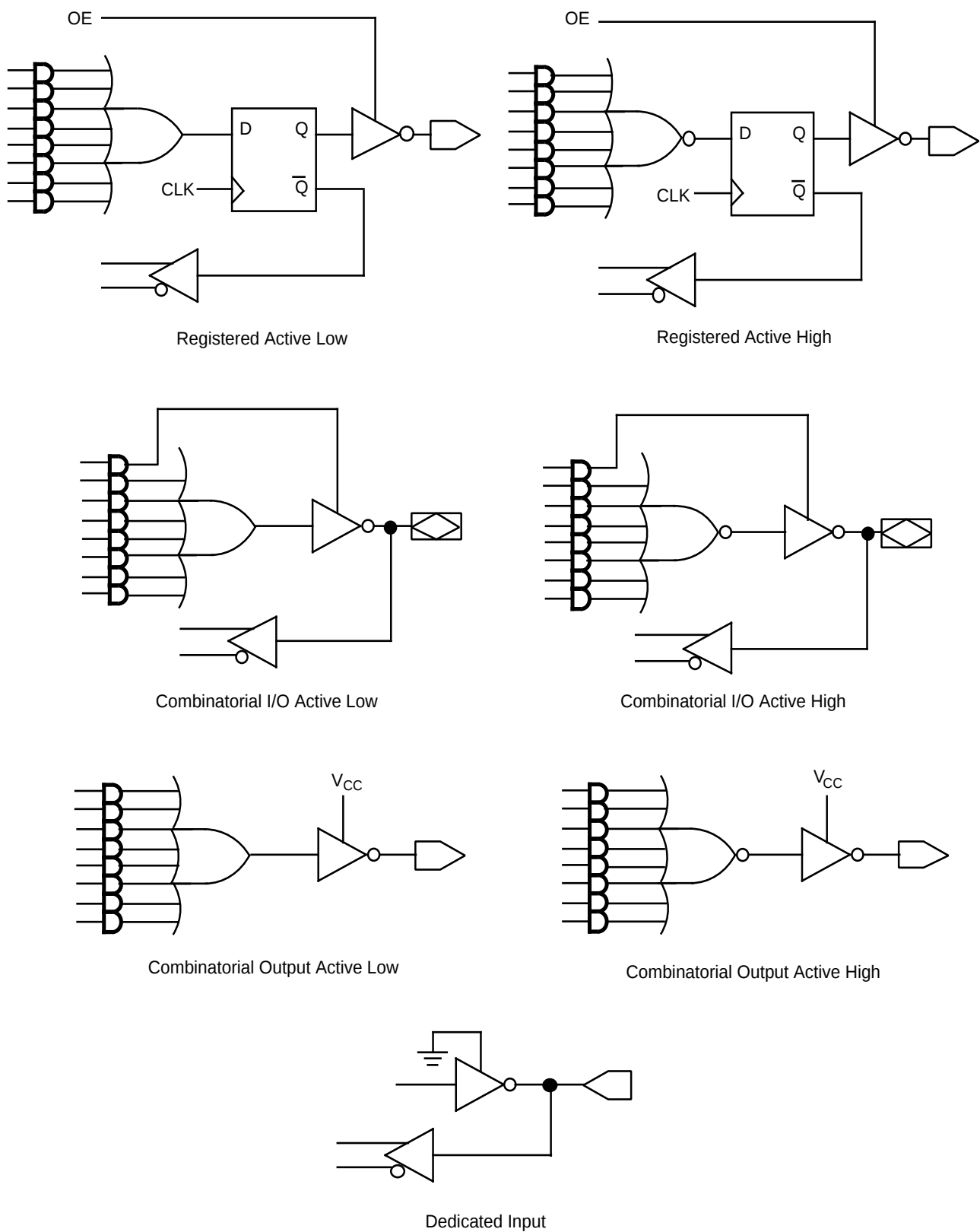
Figure 2. Macrocell Configurations
