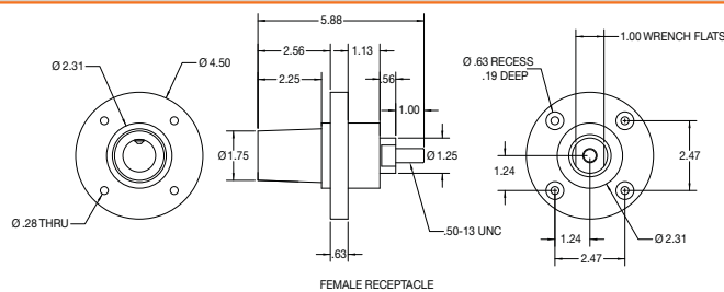
FEMALE RECEPTACLE
