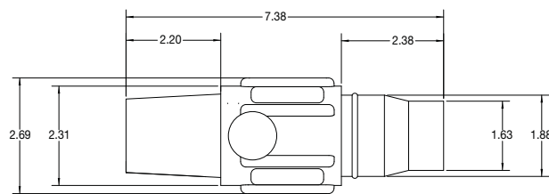
FEMALE CONNECTOR
