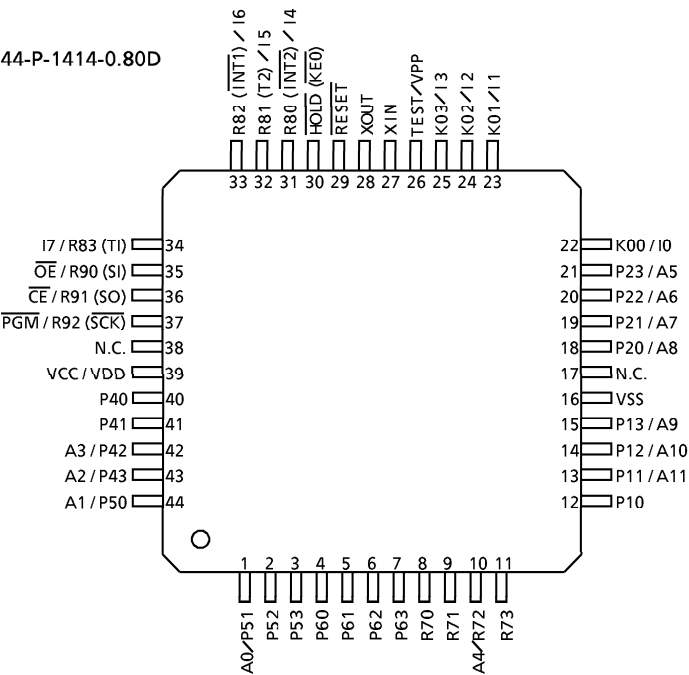
QFP44-P-1414-0.80D
