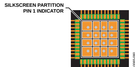
Figure 75. Typical PCB Layout
