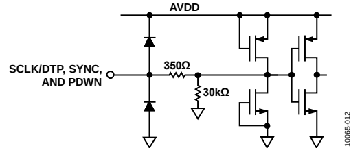
Figure 51. Equivalent SCLK/DTP, SYNC, and PDWN Input Circuit
