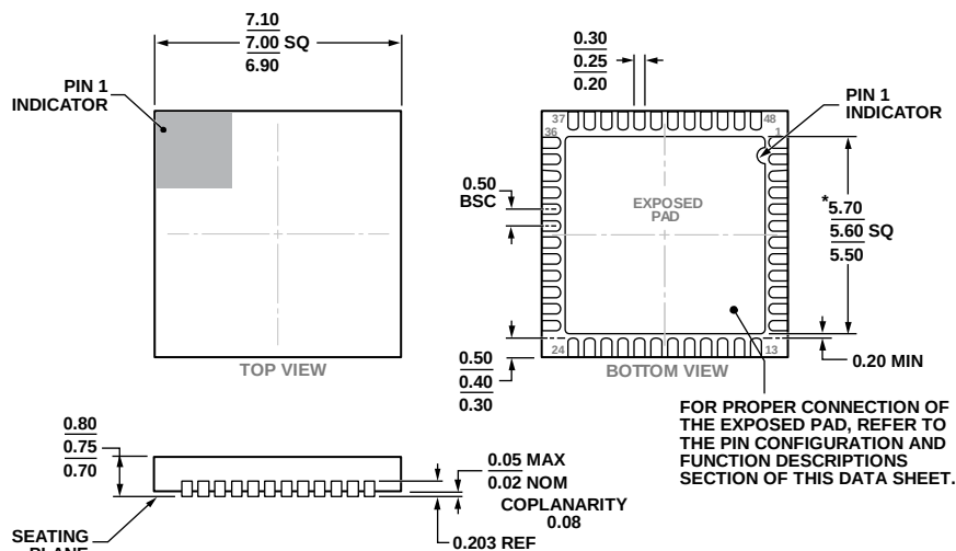
Figure 77. 48-Lead Lead Frame Chip Scale Package [LFCSP_WQ] 7 mm × 7 mm Body, Very Very Thin Quad (CP-48-13)
