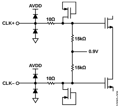
Figure 48. Equivalent Clock Input Circuit
