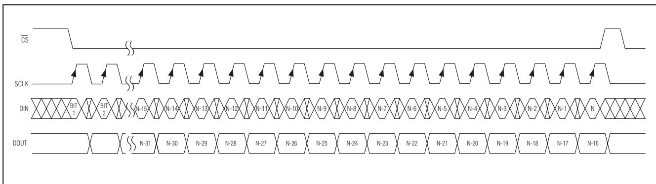
Figure 6. Transmission of More than 16 Bits to the MAX7317
