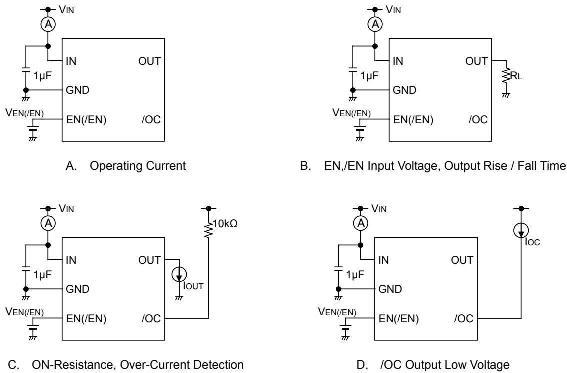
Figure 1. Measurement Circuit
