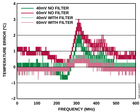
Figure 6. Temperature Error vs. Differential Mode Noise Frequency (With and Without R-C-R Filter of 100 \Omega –2.2 nF–100 \Omega )
