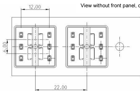
Plunger size 18 x 18 mm
