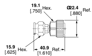
TNC Plug to 7 mm Jack
