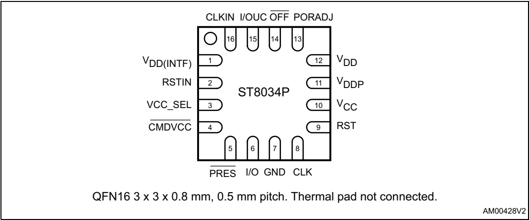
Figure 5. Pin connections ST8034P (options VCC_SEL and PORADJ pins), top-through view
