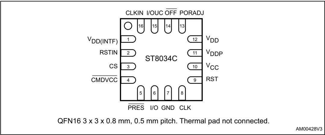
Figure 6. Pin connections ST8034C (options chip select and PORADJ pins), top-through view
