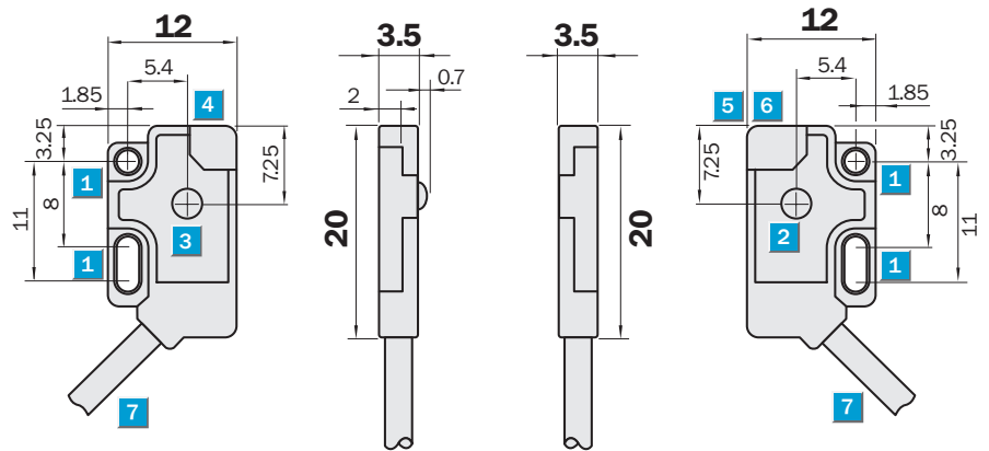
Dimensional drawing
