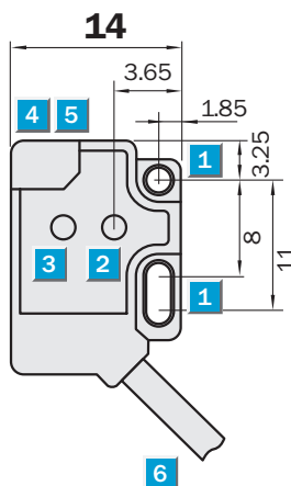
Dimensional drawing
