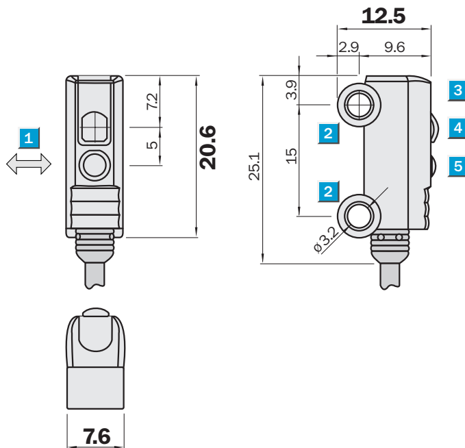
Dimensional drawing
