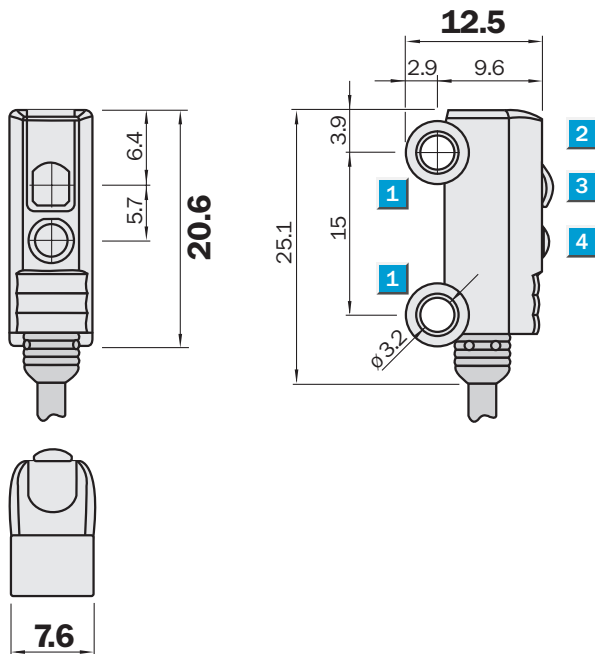
Dimensional drawing
