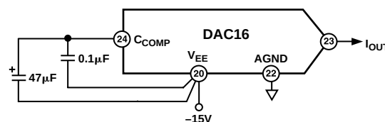
Figure 21a. Recommended Compensation Scheme to V_{EE}
