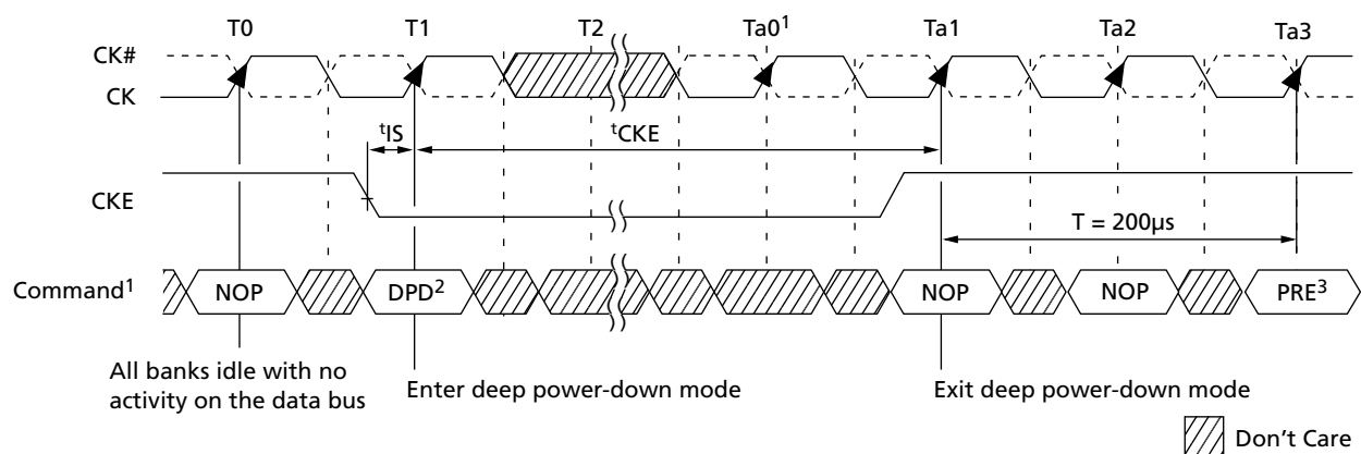
Figure 53: Deep Power-Down Mode
