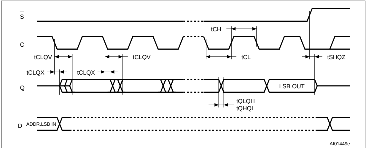
Figure 22. Output timing
