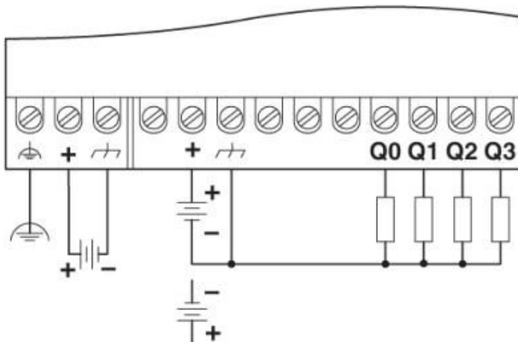
Connection diagram
