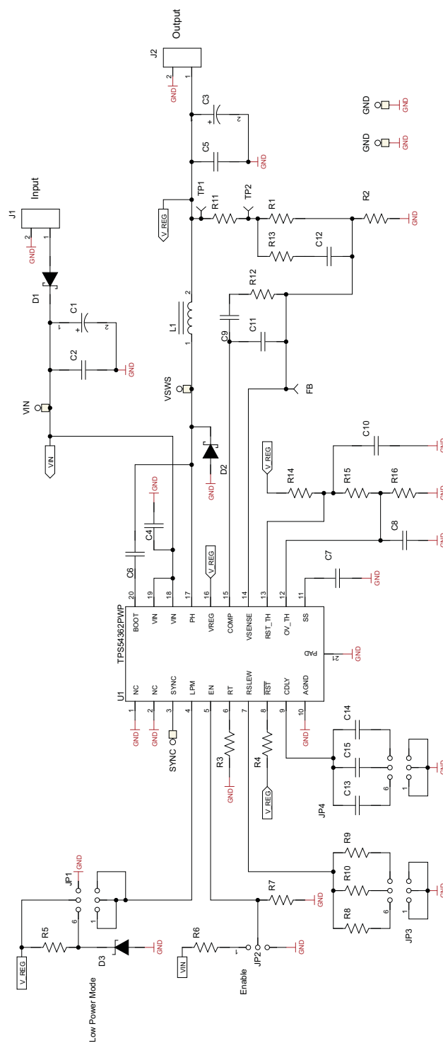
Figure 8. TPS54362EVM Schematic
