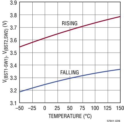
V_{(BST1-SW1)}, V_{(BST2-SW2)} UVLO vs Temperature
