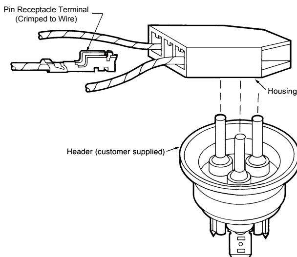
Typical Assembly
