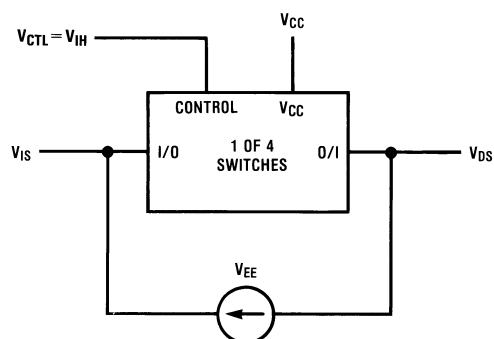
Figure 1. "ON" Resistance
