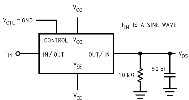
Figure 11. Sinewave Distortion
