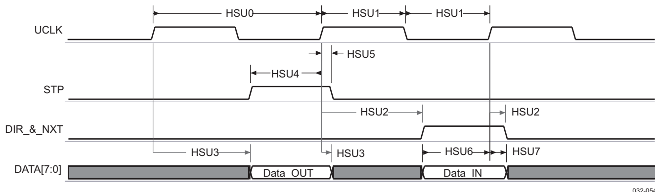
Figure 5-53. HS USB Interface—Transmit and Receive Modes (ULPI 8-Bit)
