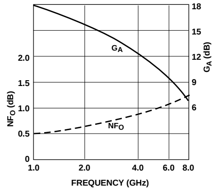
Figure 1. Optimum Noise Figure and Associated Gain vs. Frequency.
